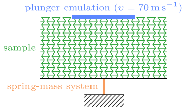
Fig. 3.6. Geometry and boundary conditions for the JIVE analyses.
