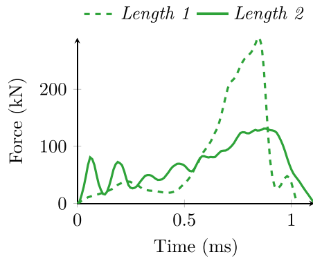
Fig. 4.3. Experimental comparison of samples sizes for ARH.
