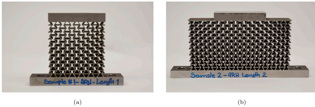
Fig. 2.3. Assembly of ARH unit cells into patches to be investigated, (a) Length 1 and (b) Length 2.
