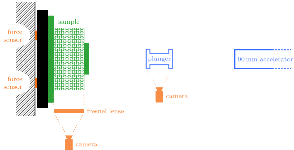
Fig. 3.1. Schematic view of the experimental set-up.
