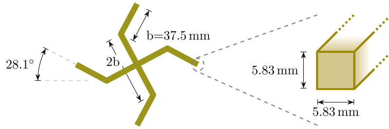
Fig. 2.2. Chiral unit cell used throughout this investigation.
